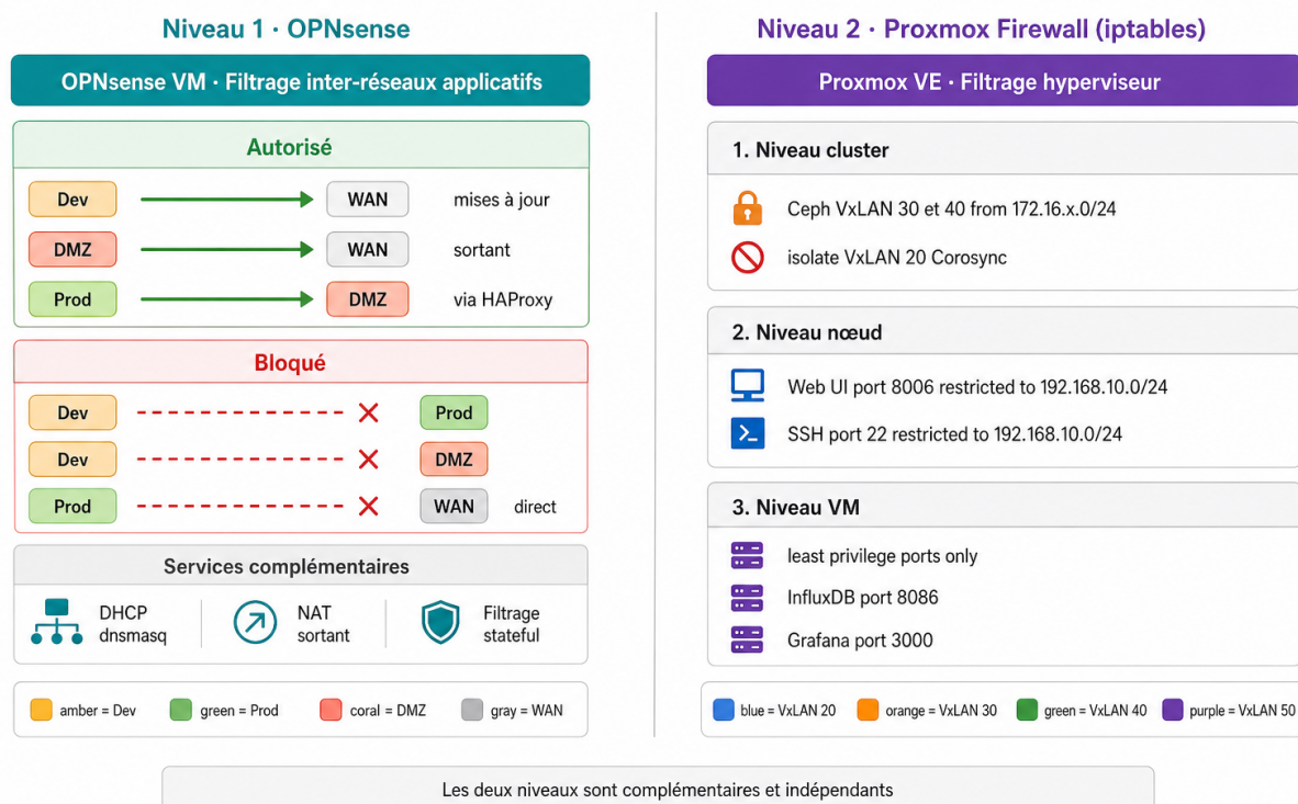
FIGURE III.5 – Architecture du Pare-feu : OPNsense et Proxmox Firewall
